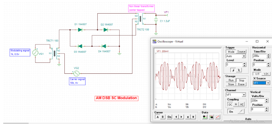
Simulation using TinaPro
